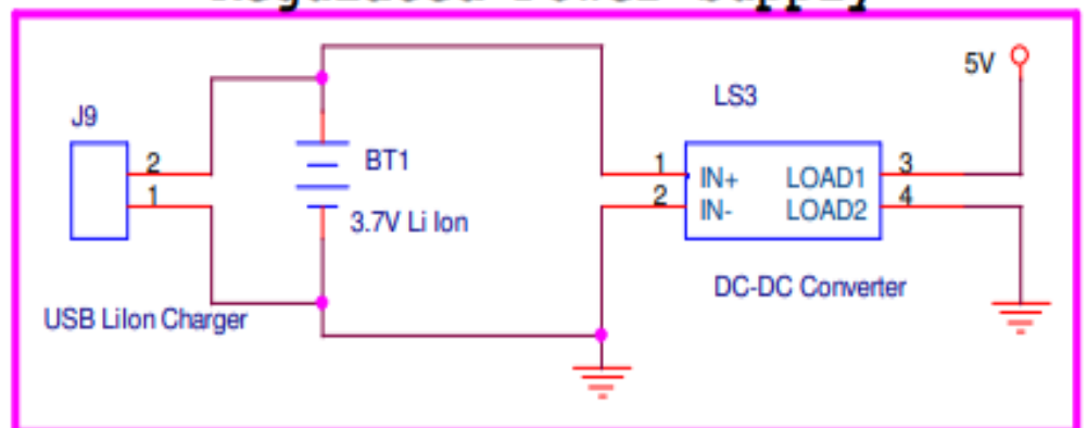
Circuit Diagram of Helmet Unit
